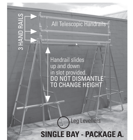
3 HAND RAILS All Telescopic Handrails Handrail slides up and down in slot provided. DO NOT DISMANTLE TO CHANGE HEIGHT Leg Levelers SINGLE BAY - PACKAGE A.
