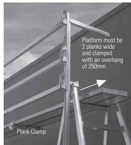
Plank Clamp
